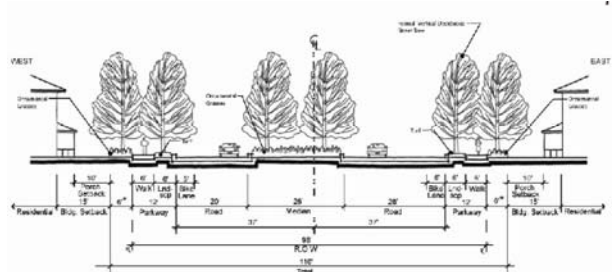
T1 Mid-block cross section Main Street Kimball Avenue to Loop Road (Bike Lane and no On-street Parking)
