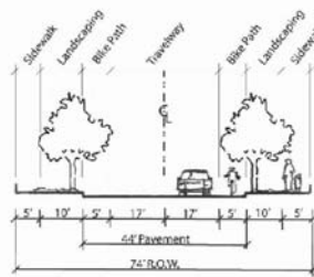
P Mid-block cross section Commercial Collector, Typical (no on-street parking)
