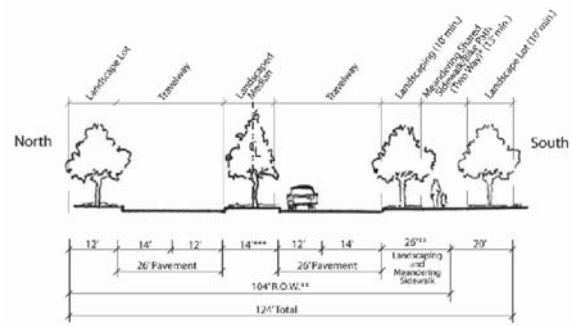
G1 Mid-block street section Major Arterial with Paseo Kimball Ave. between Euclid to Flight Avenues (no on-street parking)
