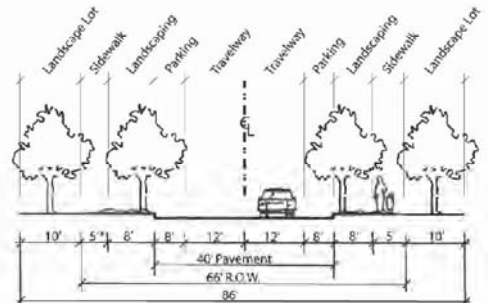
L Mid-block cross section Local Collector, Typical (with parking)
