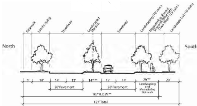
G2 Mid-block street section Major Arterial with Paseo Kimball Ave. between Flight to Hellman Avenues (no on-street parking)
