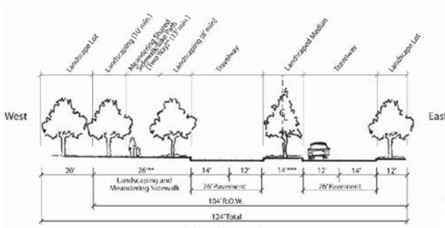
F Mid-block street section Major Arterial with Paseo Hellman from Merrill to Remington
