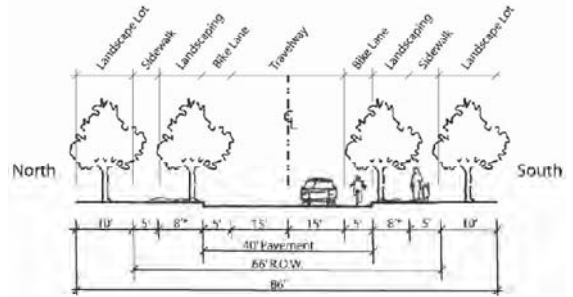
I1 Mid-block cross section Local Collector, Typical (with bike lane, no on-street parking)
