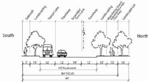
M1 Mid-block street section Local Collector with Transit & Paseo Bickmore between Euclid to Mayhew Avenues (no on-street parking)
