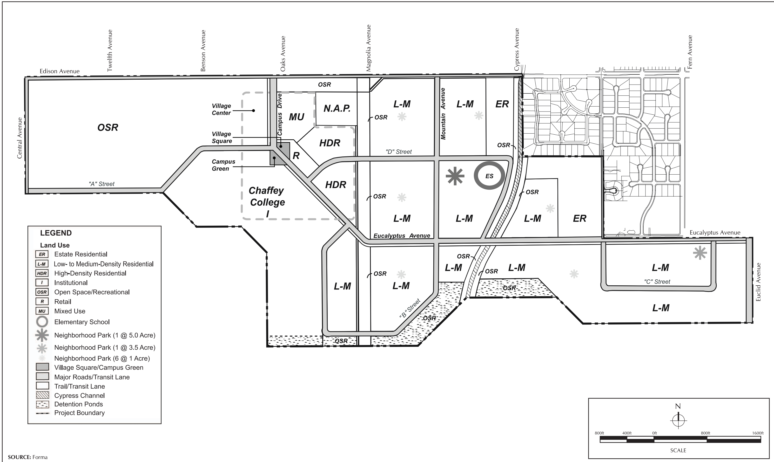
FIGURE 2.4-1 Conceptual Site Plan
